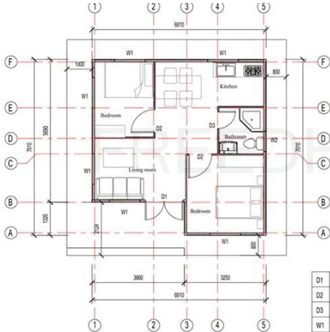
Layout plan
